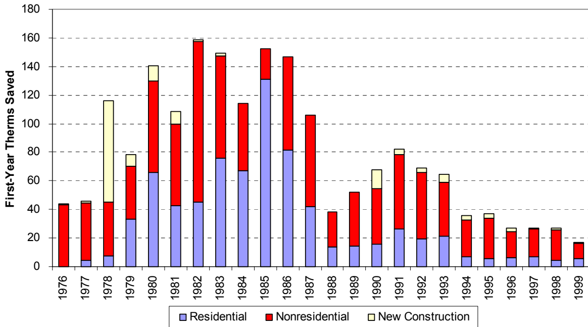
Figure 3-3 First-Year Natural Gas Savings for Major IOUs' Efficiency Programs*
