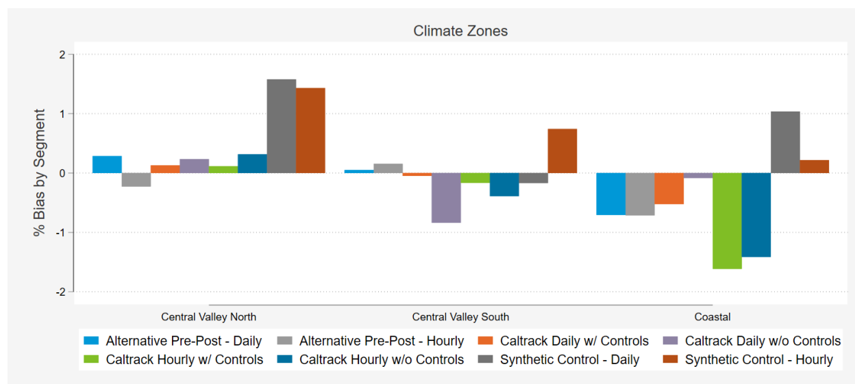
Figure 14: Residential Electric Model Results by CEC Climate Zone 15
