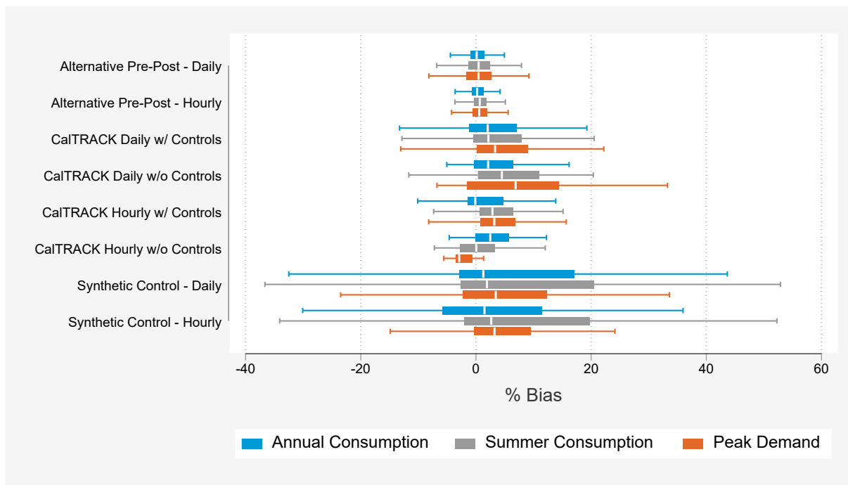
Figure 36: Distribution of Errors for Each Framework by Metrics of Interest
