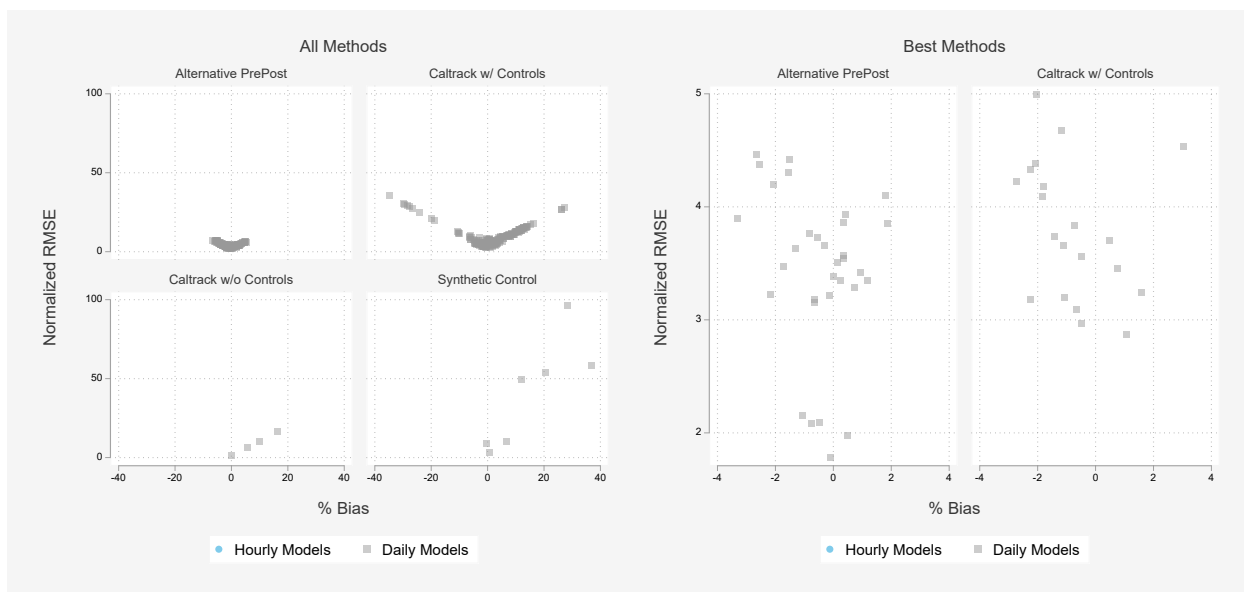
Figure 28: Overall Accuracy and Precision for Commercial Gas Models
