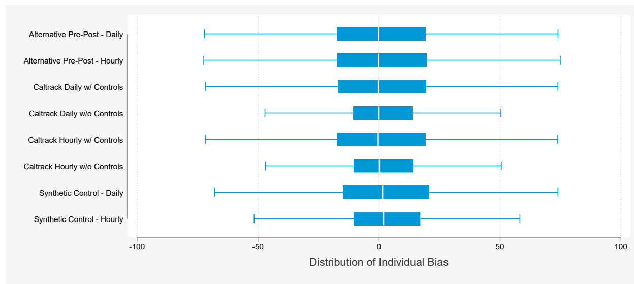
Figure 13: Residential Electric Individual Error Distribution
