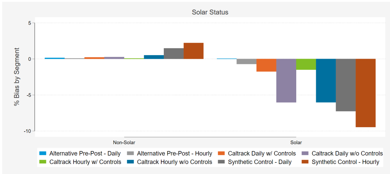
Figure 16: Residential Electric Model Results by Solar Status
