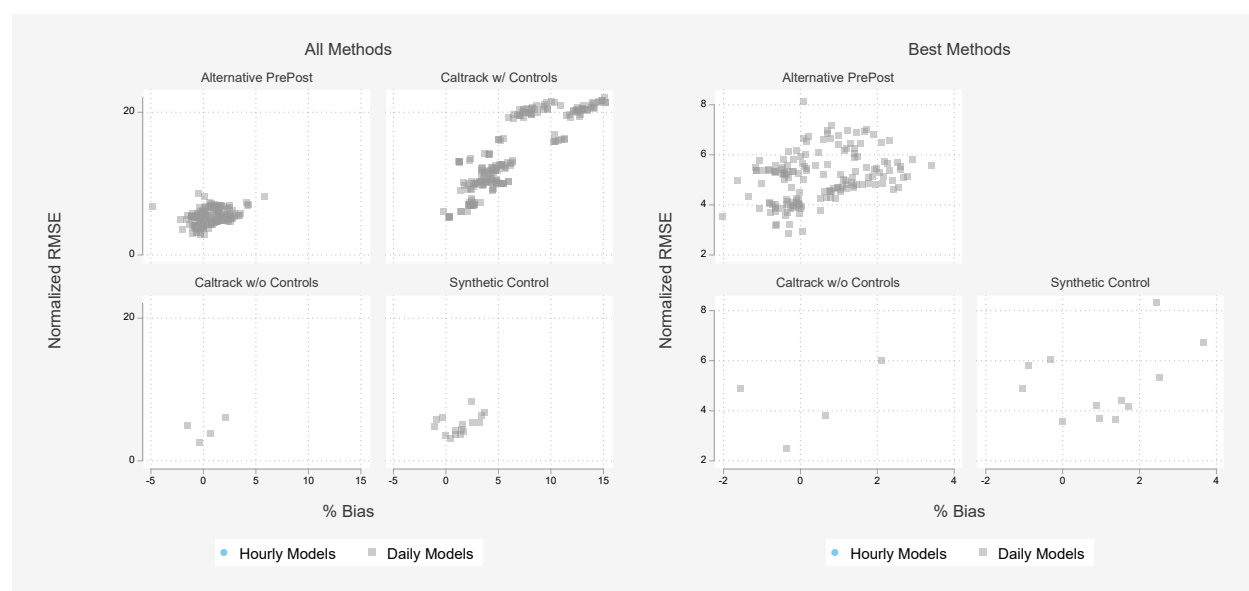
Figure 23: Overall Accuracy and Precision for Residential Gas Models
