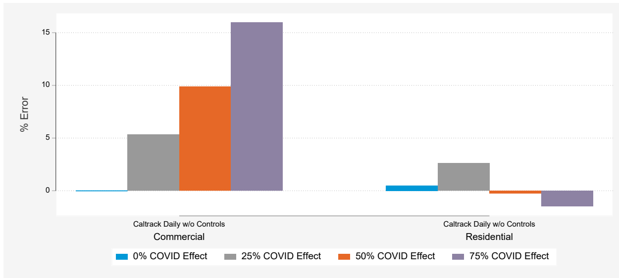
Figure 10: Errors for CalTRACK without Controls on Gas Consumption
