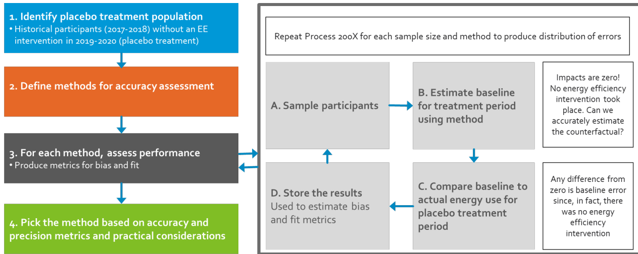
Figure 5: General Approach for Accuracy Assessment
