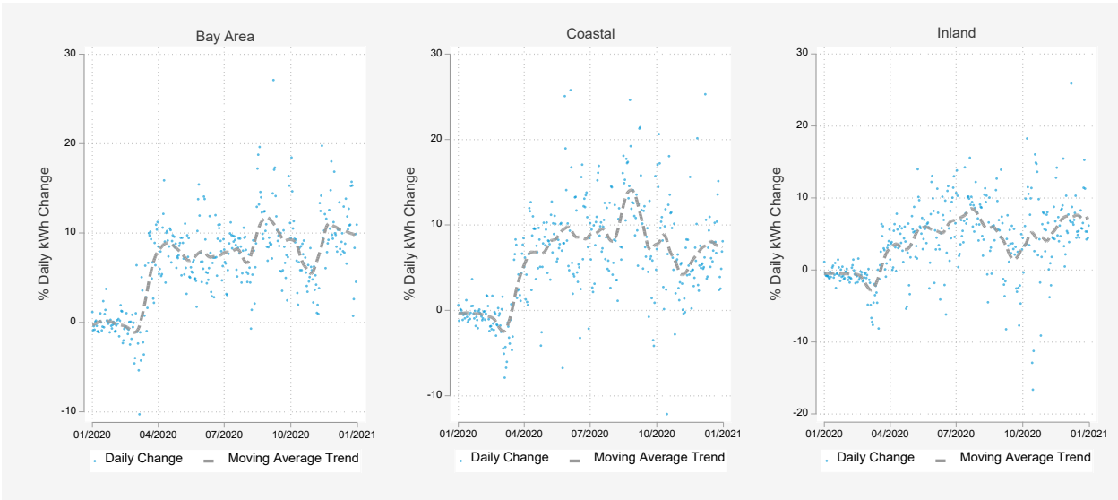
Figure 3: Residential Changes in Electricity Consumption Associated with the Pandemic
