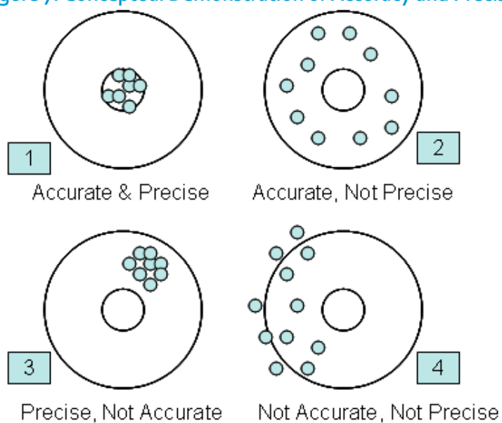
Figure 7: Conceptual Demonstration of Accuracy and Precision
