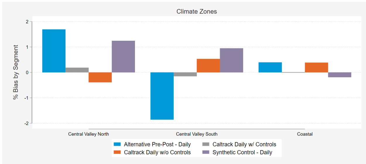
Figure 25: Residential Gas Model Results by Climate Zone 21
