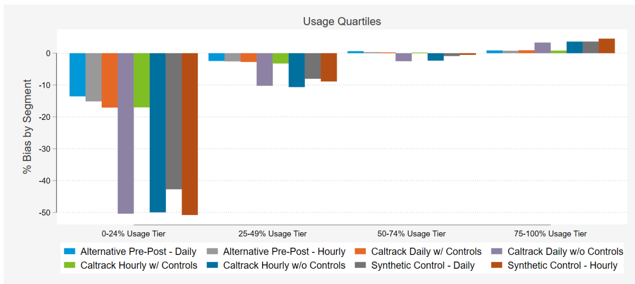
Figure 17: Residential Electric Model Results by Customer Size
