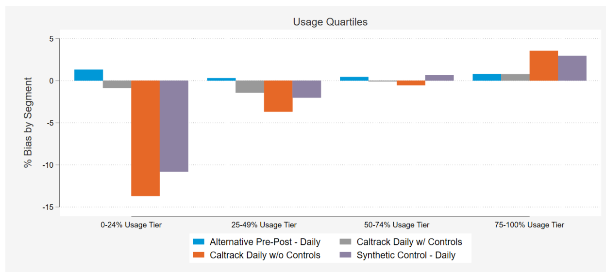
Figure 27: Residential Gas Model Results by Customer Size
