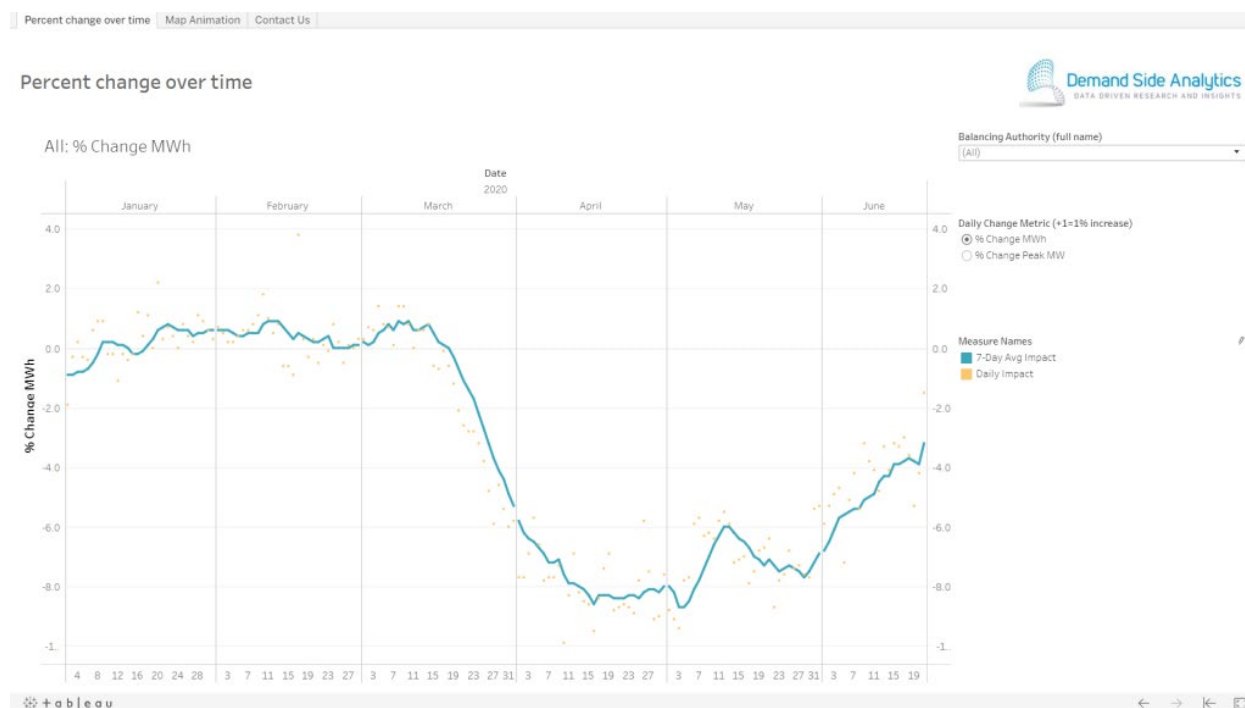
Figure 2: Electricity Consumption Changes Associated with COVID-19 Pandemic
