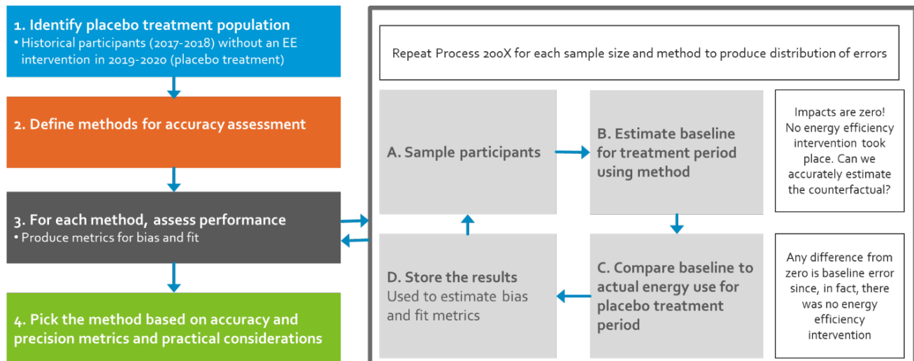
Figure 1: General Approach for Accuracy Assessment
