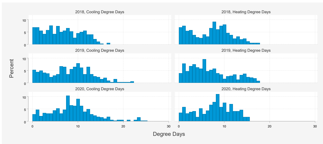
Figure 11: Distributions of Heating and Cooling Degree Days by Year
