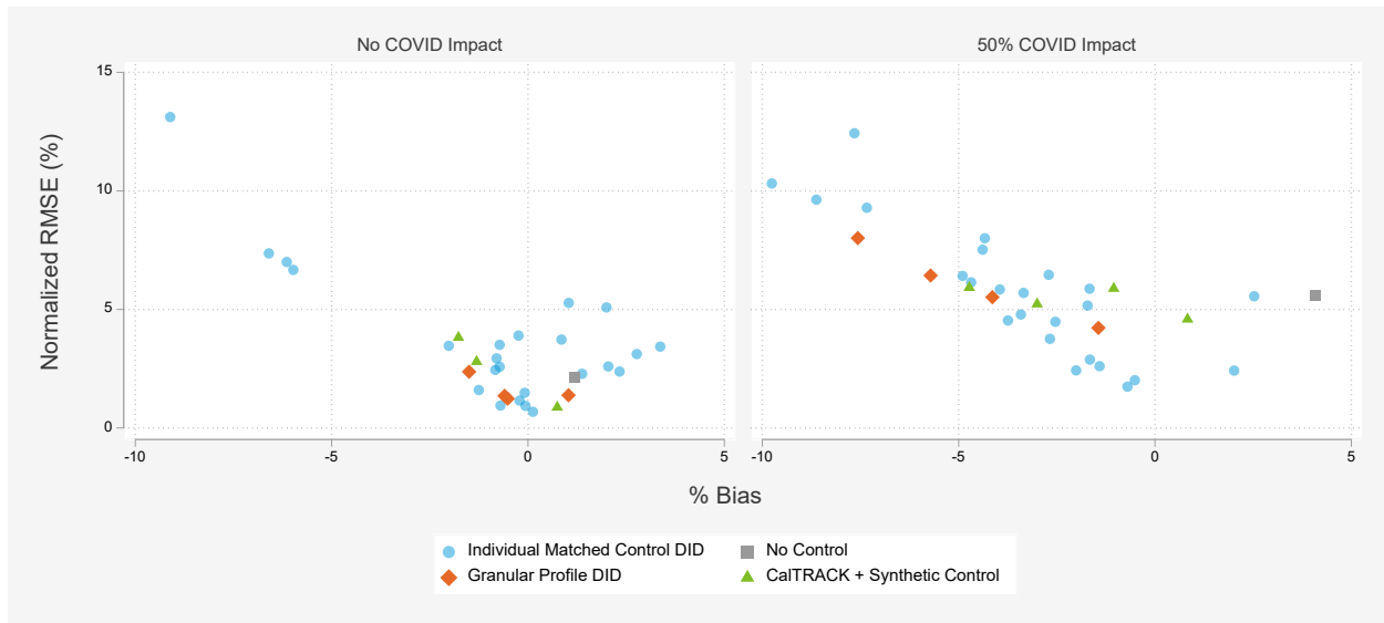
Figure 33: Commercial Electric Results for Alternative Granular Profile Tests
