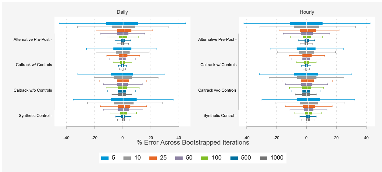
Figure 37: Distribution of Error across Bootstrapped Iterations for Residential Electric
