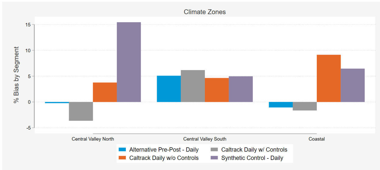
Figure 30: Commercial Gas Model Results by Climate Zone 23
