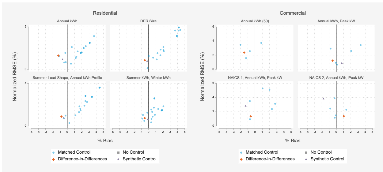
Figure 34: Comparison of Alternative Method Performance by Segmentation Strategy
