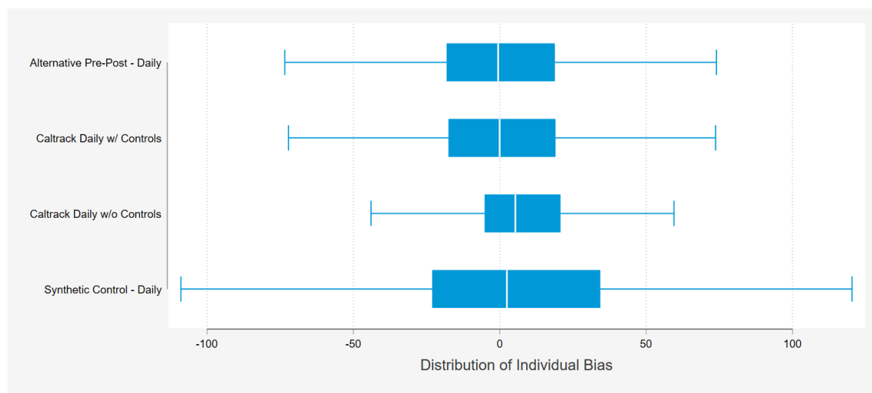
Figure 29: Commercial Gas Individual Error Distribution
