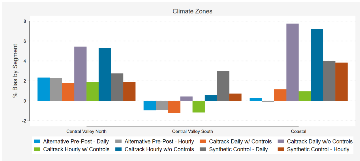
Figure 20: Commercial Electric Model Results by Climate Zone 17
