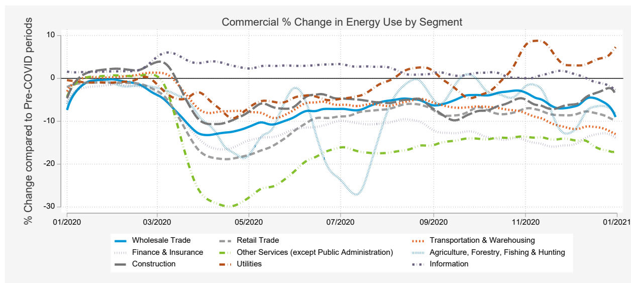
Figure 4: Commercial Changes in Energy Consumption Associated with the Pandemic
