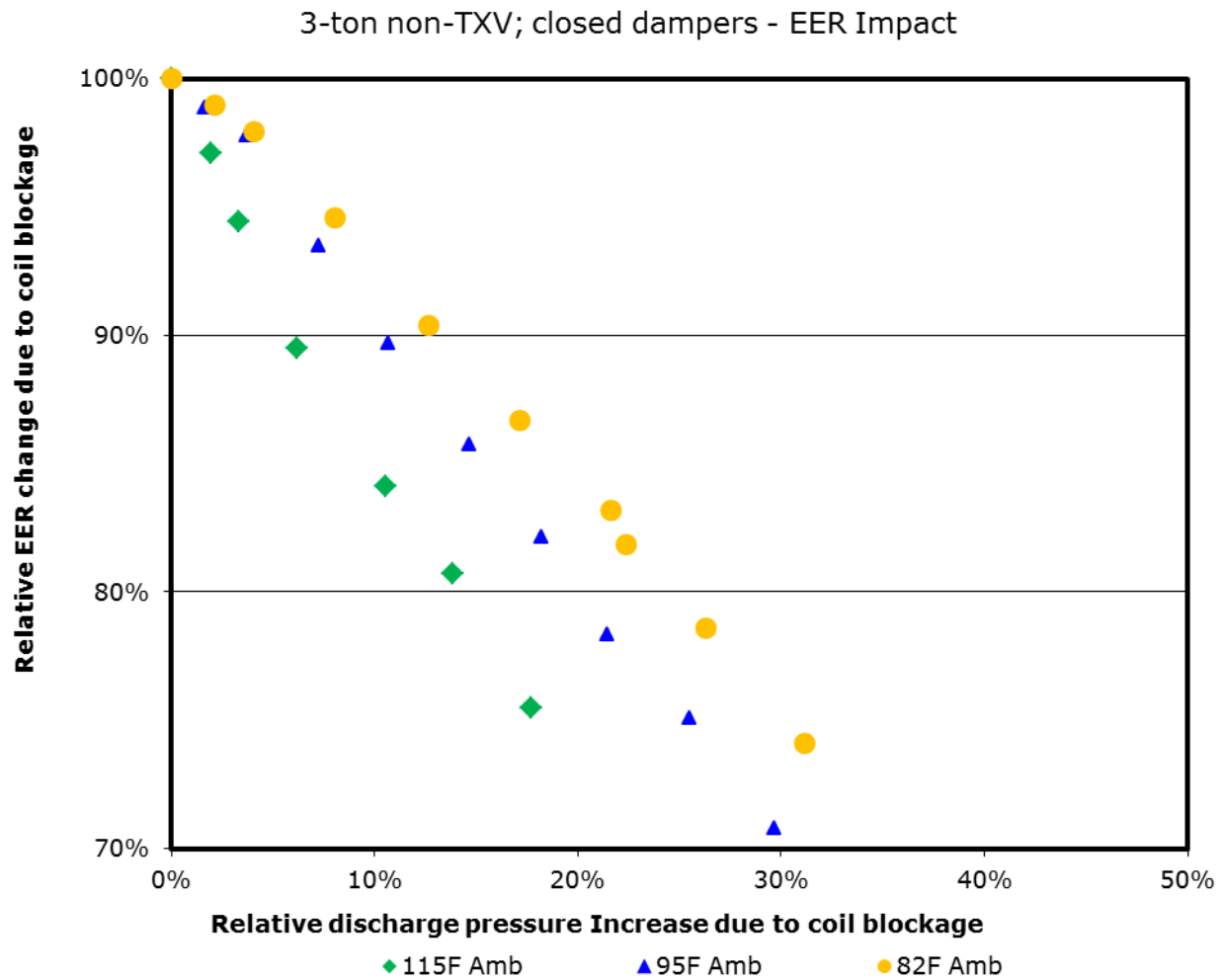
Figure 29. Relative efficiency impact due to condenser coil blockage
