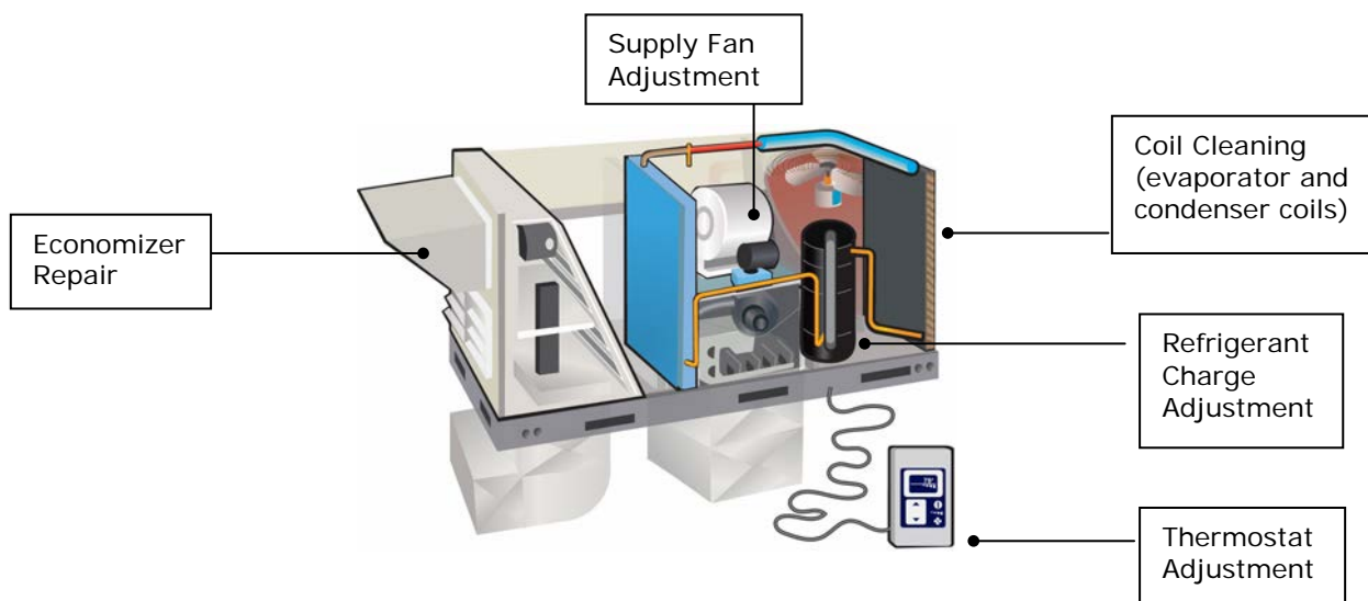
Figure 1. Schematic of a rooftop unit and location of evaluated QM measure groups
