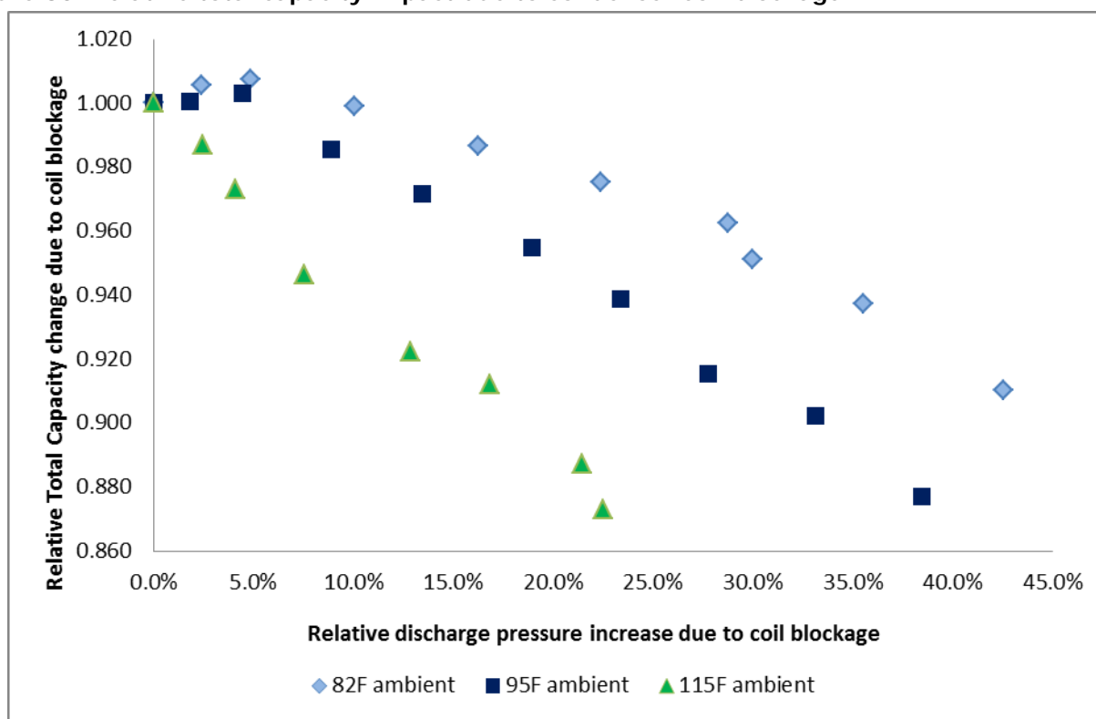
Figure 30. Relative total capacity impact due to condenser coil blockage
