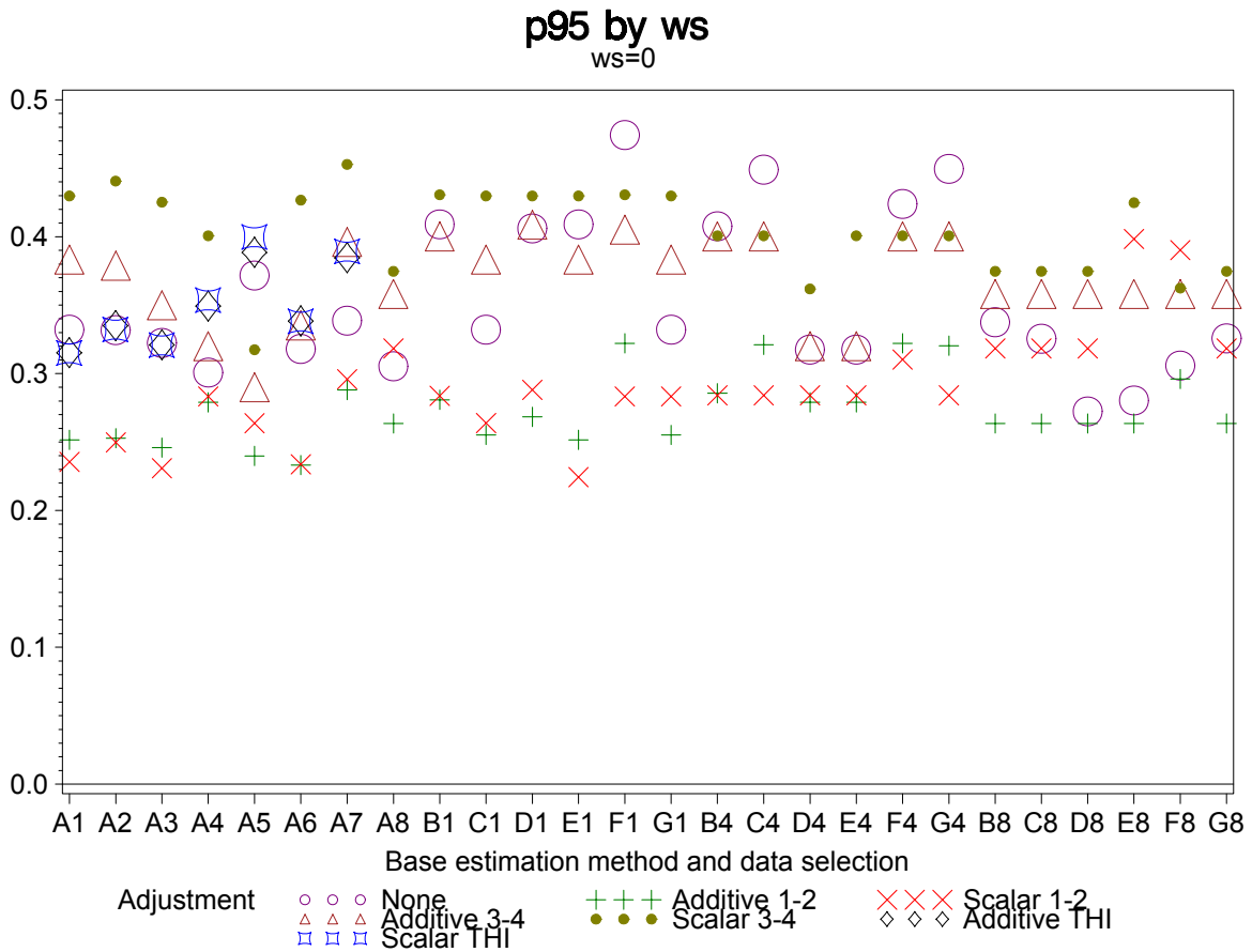
Figure 5-24 95 th Percentile Account Theil's U Nonsummer Uncurtailed Non-Weather-Sensitive Low-Variability Accounts
