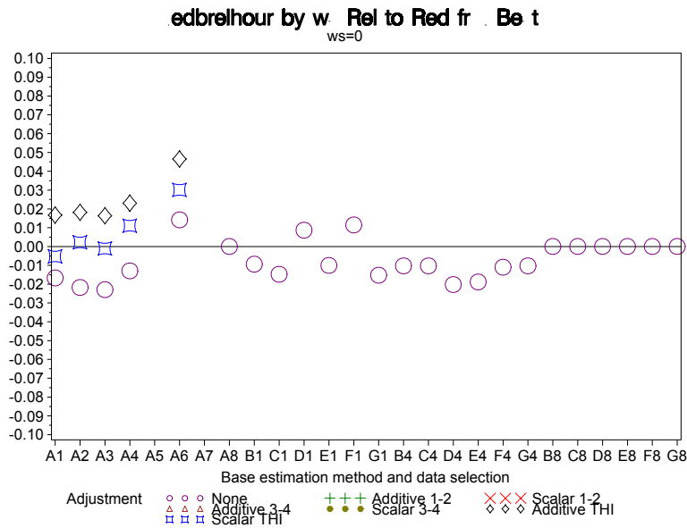
Figure B-19 Median Relative Hourly Error Nonsummer Curtailed Non-Weather-Sensitive Low-Variability Accounts
