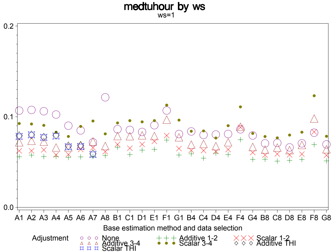
Figure 5-5 Median Account Theil's U Simple 10-Day Average and Full-Season Degree-Day Regression Summer Uncurtailed Weather-Sensitive Low-Variability Accounts
