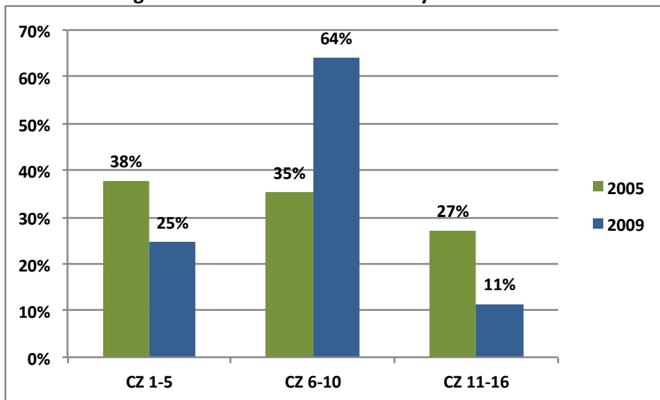
Figure 8. Insulation Installation by Climate Zone
